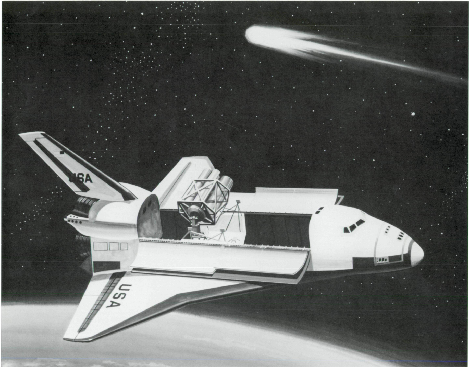
Figure 1. Observing a comet from OSS-3.
